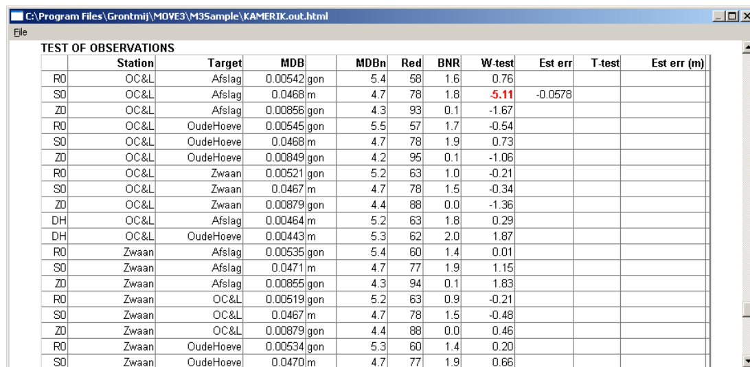
Figure 1.1-5: Test of Observations.
