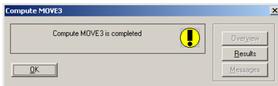
Figure 1.1-3: MOVE3 computation.
